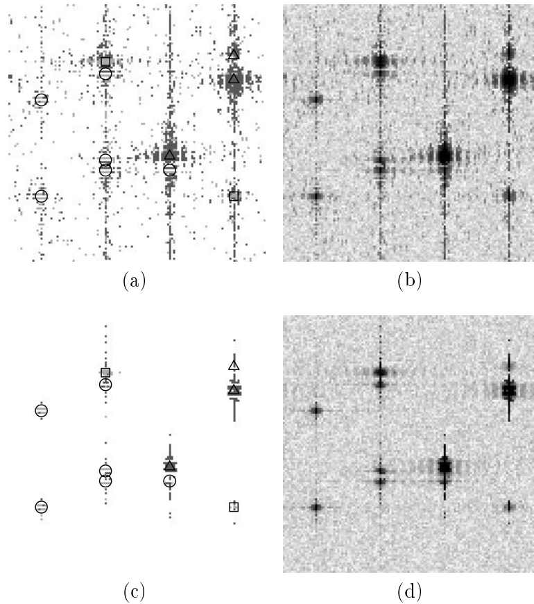
Figure 5.8. Results of using the telescopic testing procedure (a-b) with the modified GLLR and (c-d) with the MSM statistic. Images of (a,c) degree of anisotropy and (b,d) sub-aperture reflectivity.
