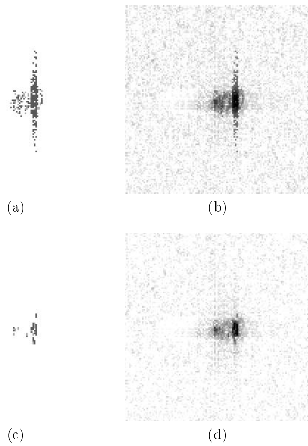
Figure 7.18. Anisotropy attributions and reflectivity images of the BMP-2 at a 0^\circ azimuth. First column: images of the anisotropy attributions. Second column: images of the associated sub-aperture reflectivities. First row: initial anisotropy attribution. Second row: fourth iteration of the anisotropy attribution.
