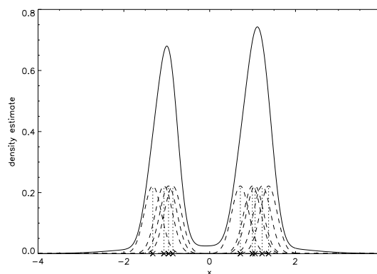
Figure 2.9. Example of Parzen density estimation.
