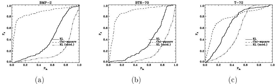
Figure 4.8. ROC detection curves for the (a) BMP-2, (b) BTR-70, and (c) T-72 using the KLD rule with \mathbf{h}_{KL} (solid curve), the \chi^2 rule with \mathbf{h}_{\chi^2} (dashed curve), and the KLD rule with \mathbf{h}_{\chi^2} (dashed-dotted curve).
