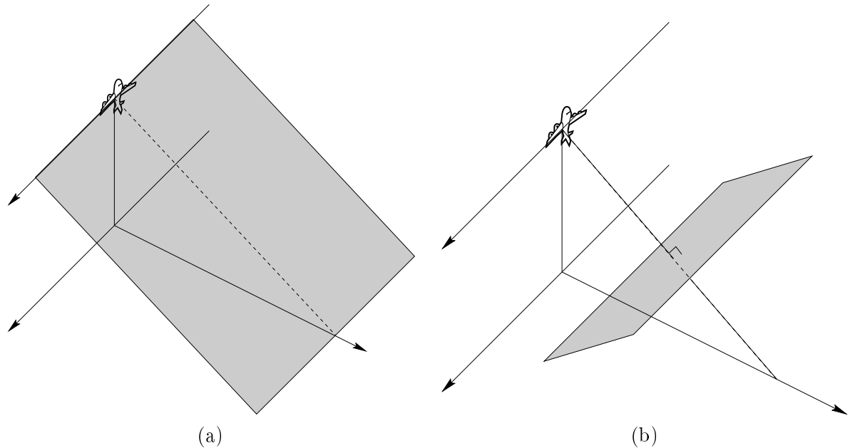
Figure 2.2. Illustration of the imaging planes (shaded region) for (a) SAR and (b) photographic imagery.
