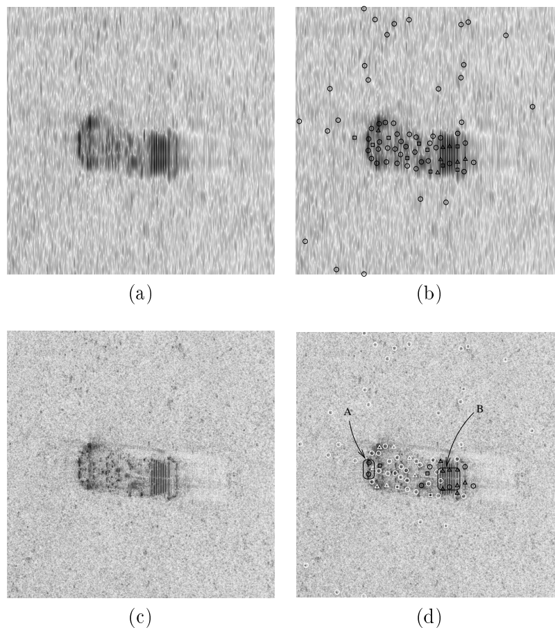
Figure 6.10. Anisotropy characterization of peaks from wide-aperture data for vehicle 1. (a) Narrow-aperture log-magnitude image. (b) Narrow-aperture image with anisotropy overlays. (c) Wide-aperture log-magnitude image. (d) Wide-aperture image with anisotropy overlays.
