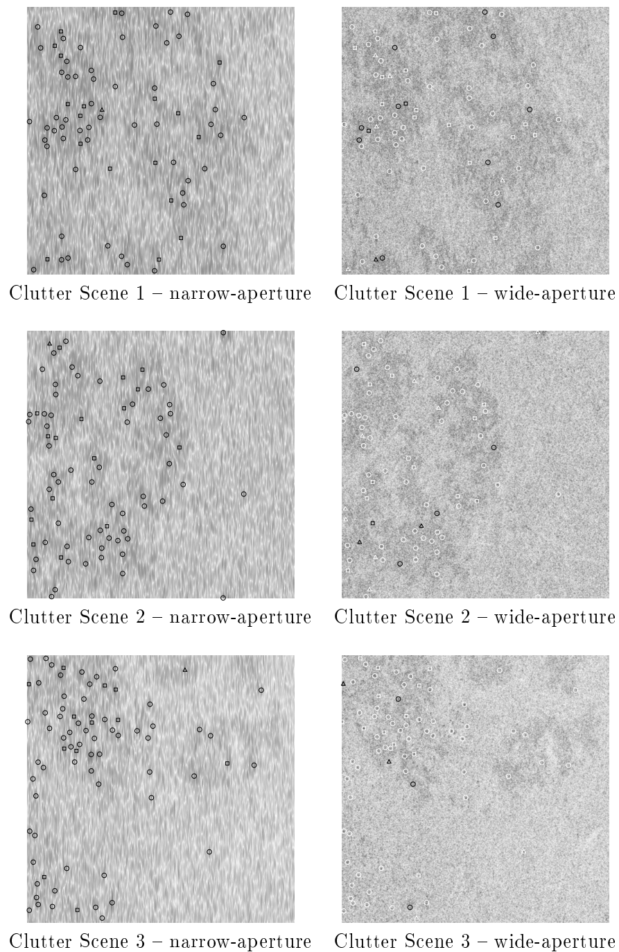
Figure 6.12. Anisotropy characterization of peaks from 3 instances of clutter in the GUS data. Left: Narrow-aperture anisotropy attributions. Right: Wide-aperture anisotropy attributions.
