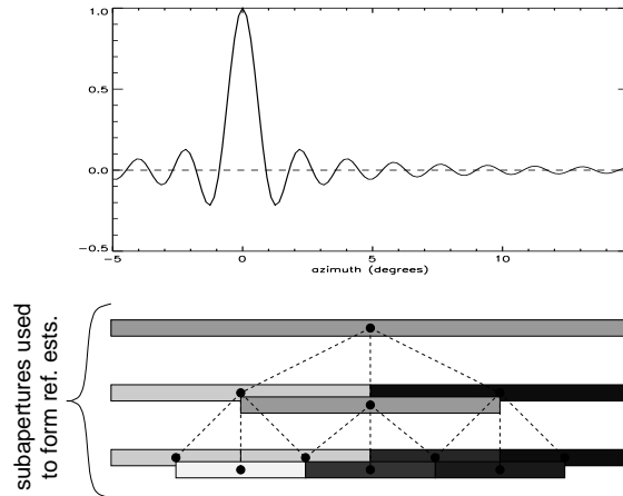
Figure 3.4. The response of a 1m \times 1m flat plate and a depiction of the reflectivity estimate for each of the sub-apertures. Lighter shaded sub-apertures convey larger reflectivity estimates.
