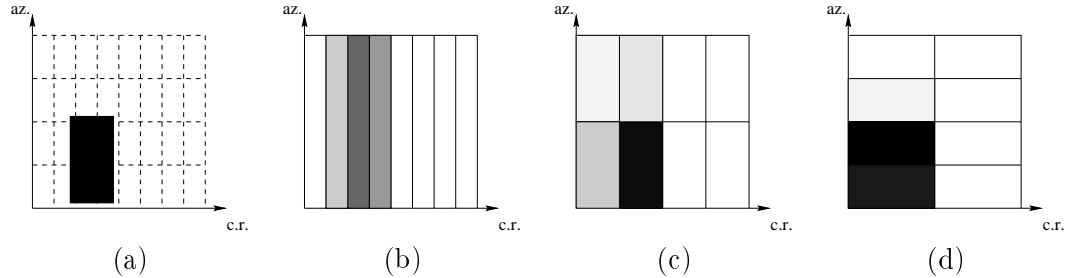
Figure 3.7. Tilings of the azimuth-cross-range plane and how they represent a distributed scatterer. (a) The underlying scatterer’s energy coverage in azimuth and cross-range. (b) Full-aperture representation. (c) Half-aperture representation. (d) Quarter-aperture representation.
