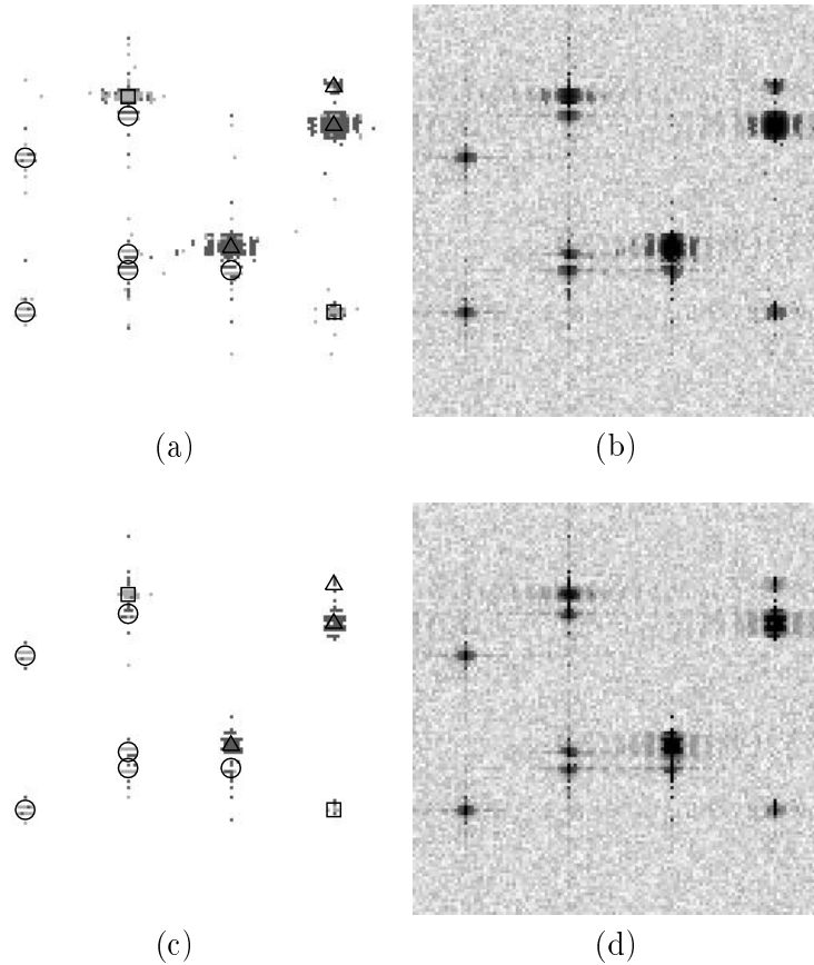
Figure 5.9. Results of using the telescopic testing procedure and a pre-screening threshold (a-b) with the modified GLLR and (c-d) with the MSM statistic. Images of (a,c) degree of anisotropy and (b,d) sub-aperture reflectivity.
