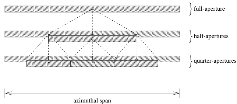
Figure 3.1. Illustration of a sub-aperture pyramid.
