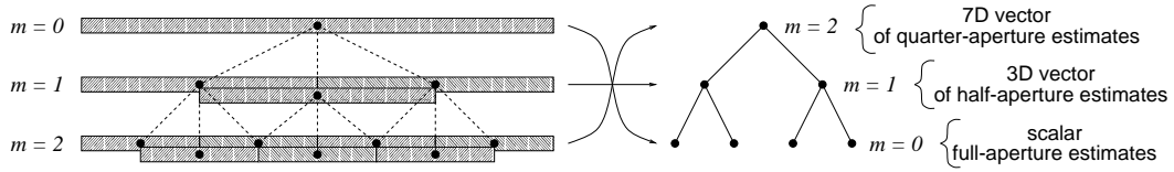
Figure 4.2. The relationship between (left) the half-overlapping, half-aperture sub-aperture pyramid and (right) the corresponding feature vector tree.
