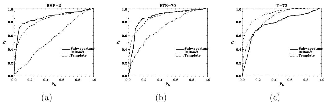
Figure 4.9. ROC detection curves for the (a) BMP-2, (b) BTR-70, and (c) T-72 using the \chi^2 rule with \mathbf{h}_{\chi^2} (solid curve), DeBonet’s algorithm (dashed curve), and the WPAFB template matching algorithm (dashed-dotted curve).
