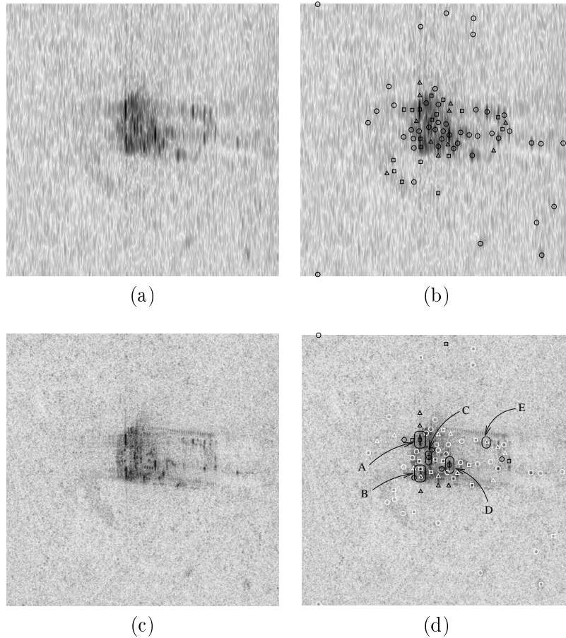
Figure 6.11. Anisotropy characterization of peaks from wide-aperture data for vehicle 2. (a) Narrow-aperture log-magnitude image. (b) Narrow-aperture image with anisotropy overlays. (c) Wide-aperture log-magnitude image. (d) Wide-aperture image with anisotropy overlays.
