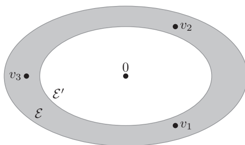
FIG. 4.1. The ellipsoids shown are \mathcal{E} = \mathcal{E}_1(v_1, v_2, v_3) and \mathcal{E}' = \mathcal{E}_{1/2}(v_1, v_2, v_3) . There is an ellipsoid passing through v_1, v_2 , and v_3 because the points are sandwiched between \mathcal{E} and \mathcal{E}' .
