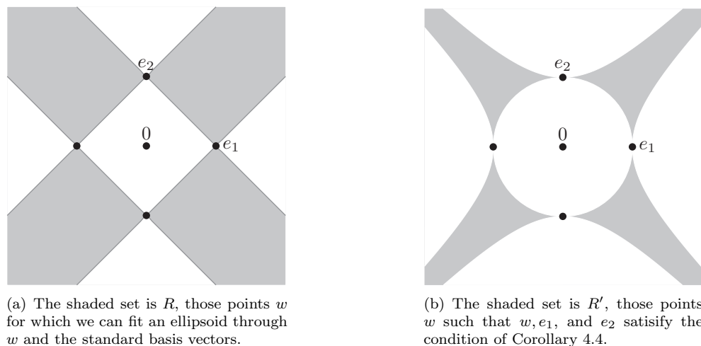
FIG. 4.2. Comparing our sufficient condition (Corollary 4.4) with the characterization (Corollary 3.7) in the case of fitting an ellipsoid to k+1 points in \mathbb{R}^k .
